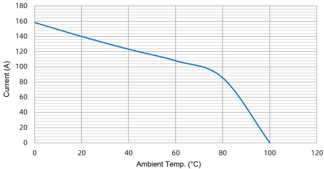
SKT 150 A Current Carrying Capacity
