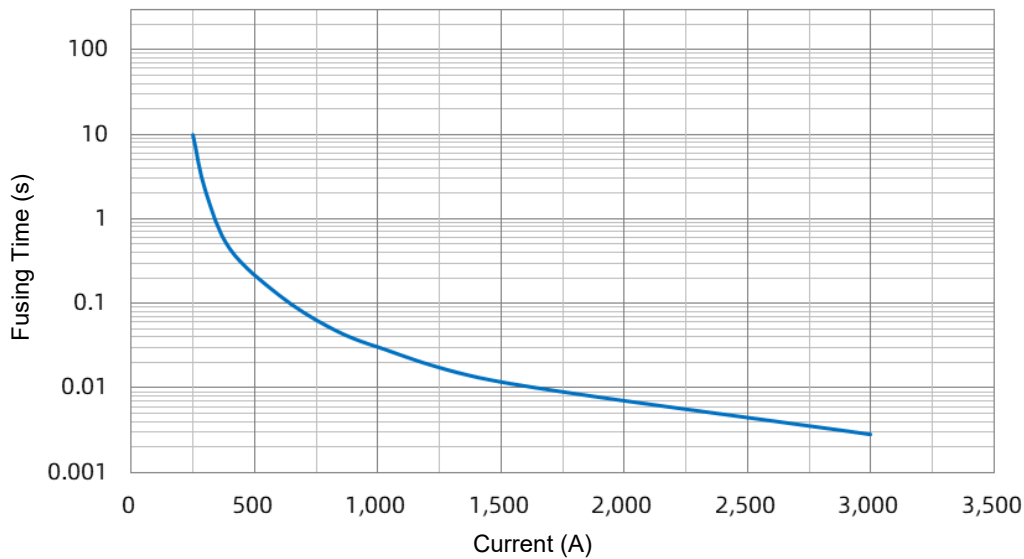
SKT 150 A Current-Time Curve
