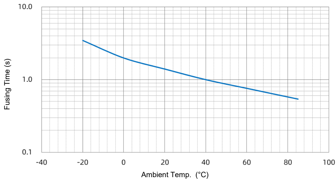
SKT 150 A Temp.-Time Curve
