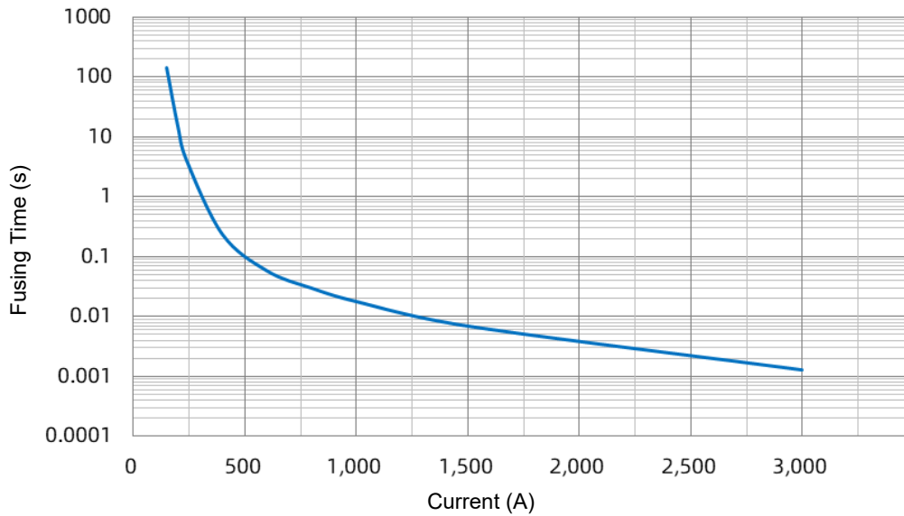
SKT 120 A Current-Time Curve
