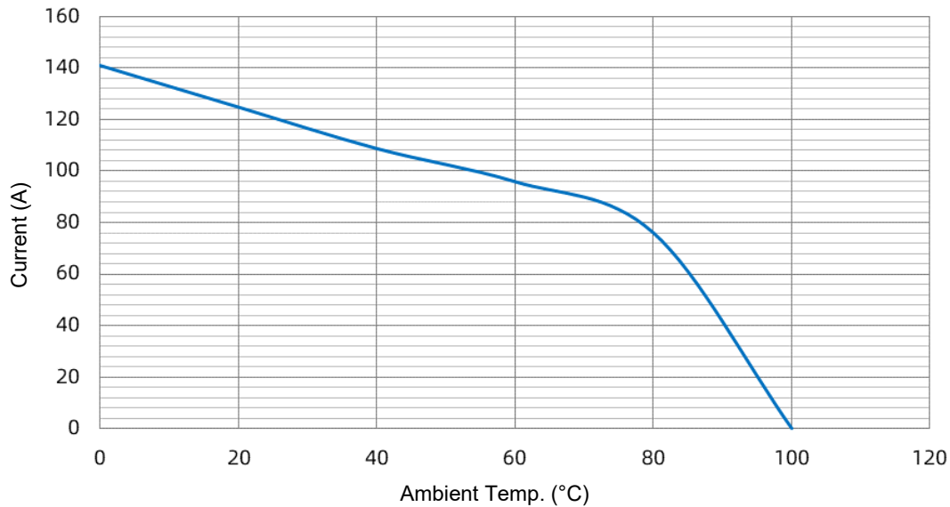
SKT 120 A Current Carrying Capacity
