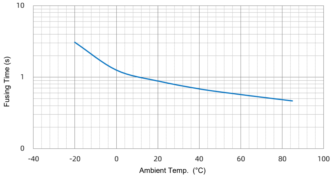
SKT 120 A Temp.-Time Curve
