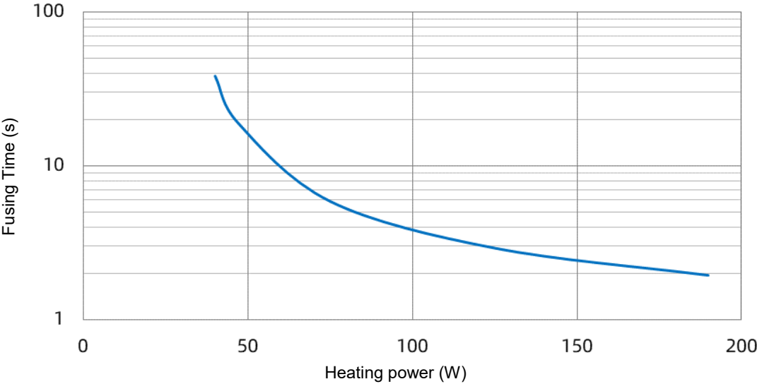
SKT 150 A Power-Time Curve
