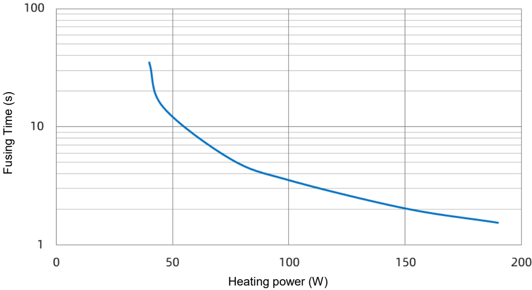
SKT 120 A Power-Time Curve
